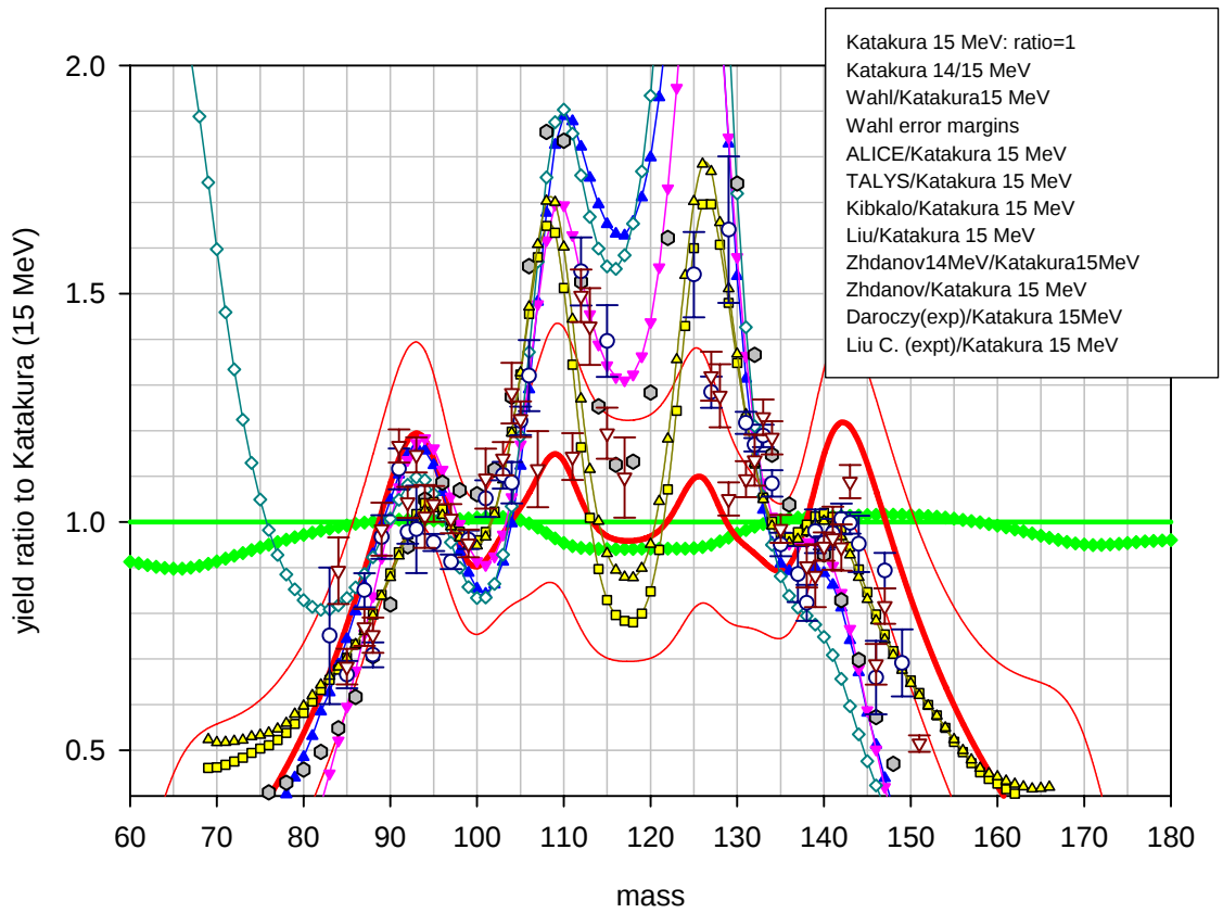
Benchmark A: ^{238}\text{U} at 14-15 MeV: post neutron emission yield ratio to Katakura's systematics at 15 MeV lower graph: partial plot (very high and low values omitted).
